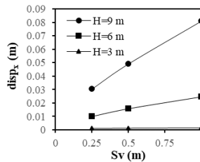
Fig 6. Horizontal wall displacement ( \text{disp}_x ) vs. vertical geo-reinforcement spacing S_v
