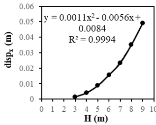
Fig 5. Horizontal wall displacement ( \text{disp}_x ) vs. wall-height H
