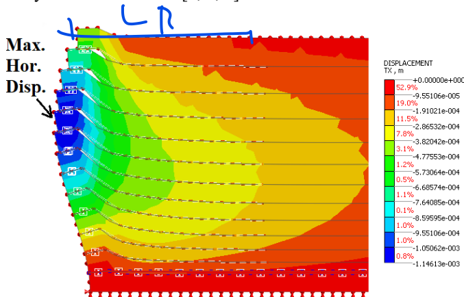
Fig. 3. Typical horizontal displacement plot in a 3 m high wall
