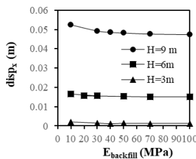
Fig 7. Horizontal wall displacement ( \text{disp}_x ) vs modulus of elasticity of the backfill ( E_{\text{backfill}} )
