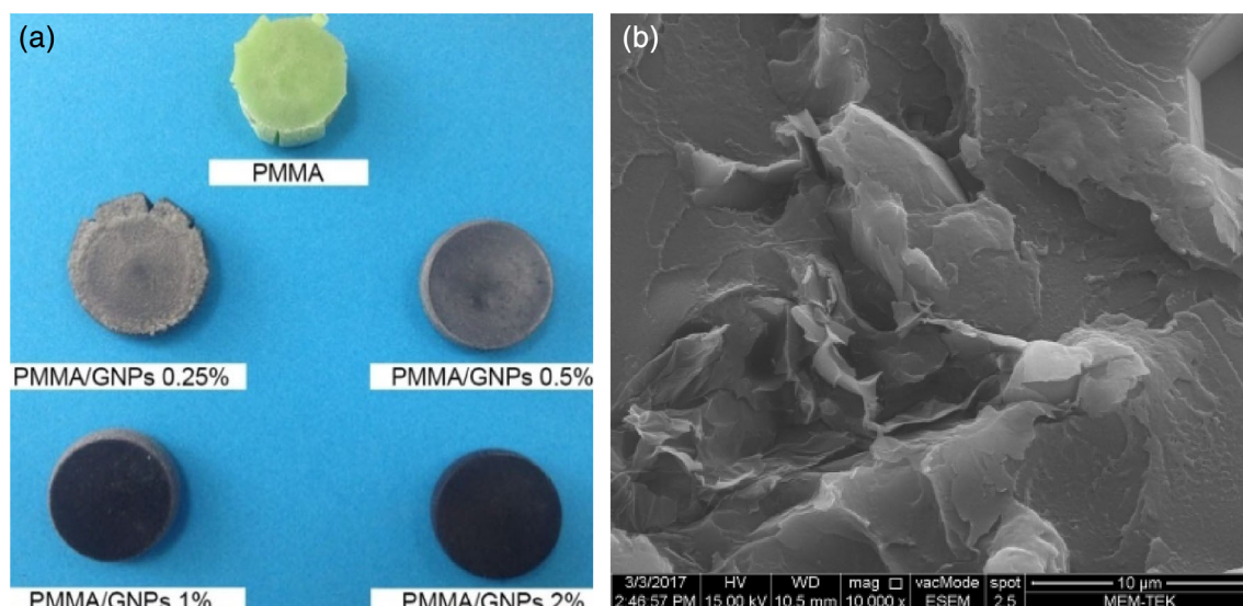
FIGURE 5 The images of poly (methyl methacrylate) (PMMA)/graphene nanoplatelets (GNPs) nanocomposite samples after the compression test [Color figure can be viewed at wileyonlinelibrary.com]
