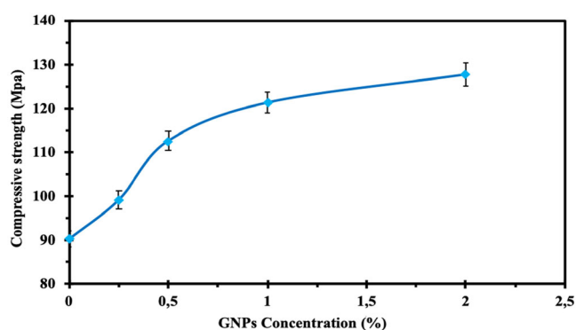
FIGURE 6 The changes in compressive strength of poly (methyl methacrylate) (PMMA)/graphene nanoplatelets (GNPs) nanocomposites [Color figure can be viewed at wileyonlinelibrary.com]
