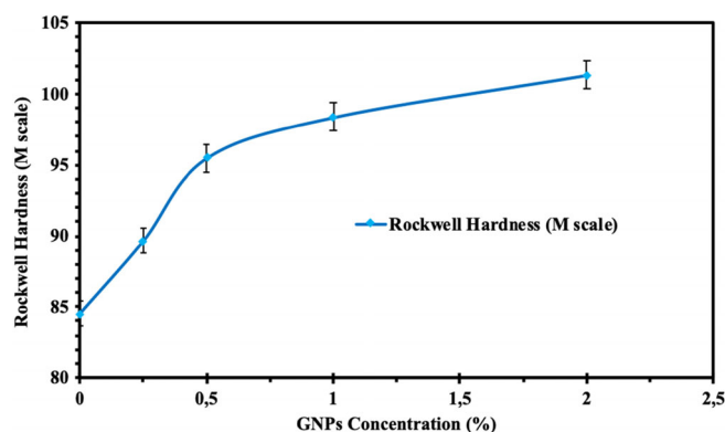
FIGURE 4 Rockwell hardness values of poly (methyl methacrylate) (PMMA)/graphene nanoplatelets (GNPs) nanocomposites [Color figure can be viewed at wileyonlinelibrary.com ]
