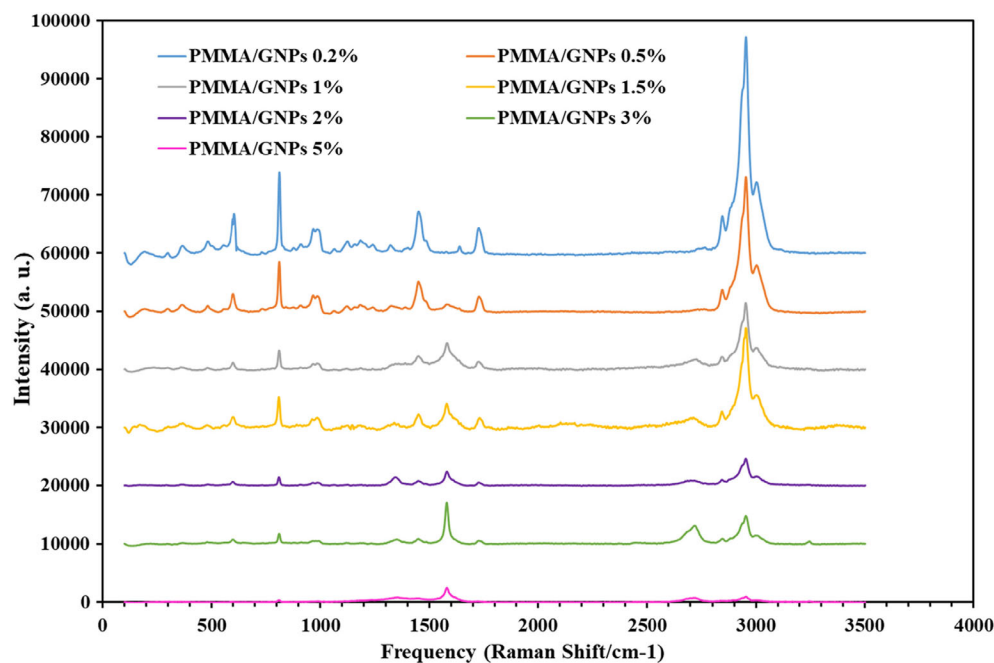
FIGURE 7 Raman spectra of the poly (methyl methacrylate) (PMMA)/ graphene nanoplatelets (GNPs) nanocomposite samples [Color figure can be viewed at wileyonlinelibrary.com ]
