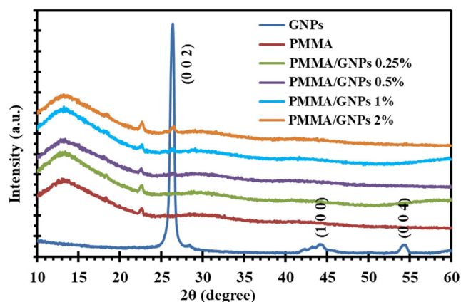
FIGURE 3 XRD patterns of poly (methyl methacrylate) (PMMA), graphene nanoplatelets (GNPs) and PMMA/GNPs nanocomposites [Color figure can be viewed at wileyonlinelibrary.com]
