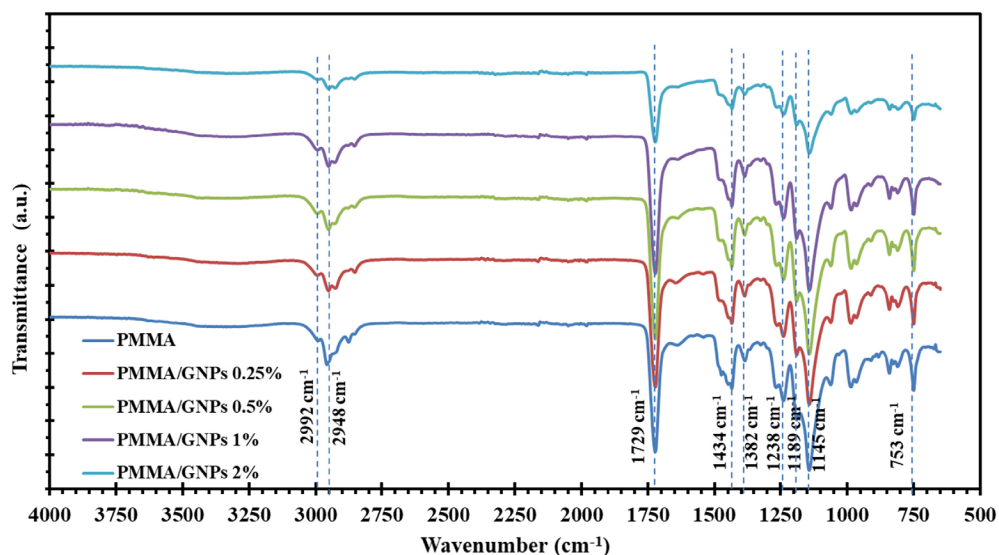
FIGURE 2 Fourier transform infrared (FTIR) spectra of pure poly (methyl methacrylate) (PMMA) and PMMA/graphene nanoplatelets (GNPs) nanocomposites [Color figure can be viewed at wileyonlinelibrary.com]
